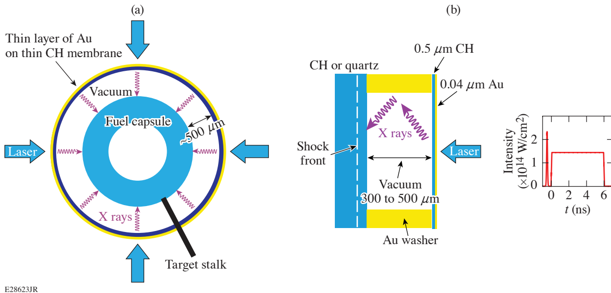
Figure 1 Schematic of (a) the spherical hybrid direct-drive target design and (b) the planar target design that was tested in the experiment.
