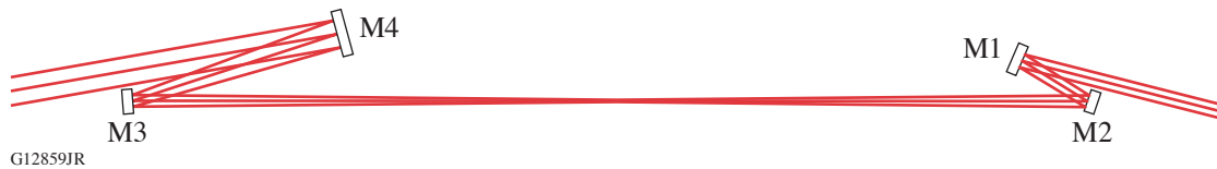
Figure 1 The final layout of the AIR mirrors, showing the ray path from the central field point.
